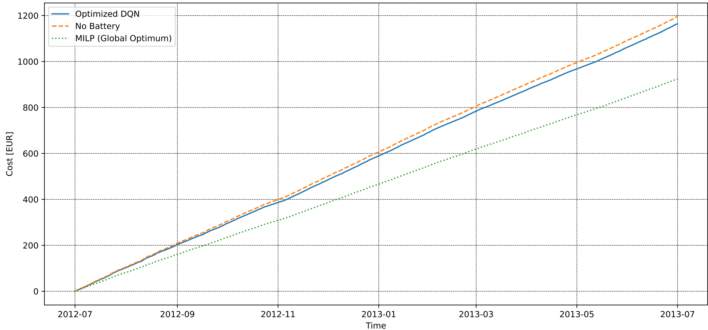
User 127 - Basic Training - Electricity Cost [DQN vs MILP]
